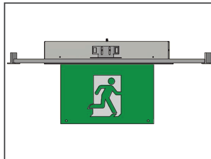
Ceiling Recessed Mounting, See page 6
